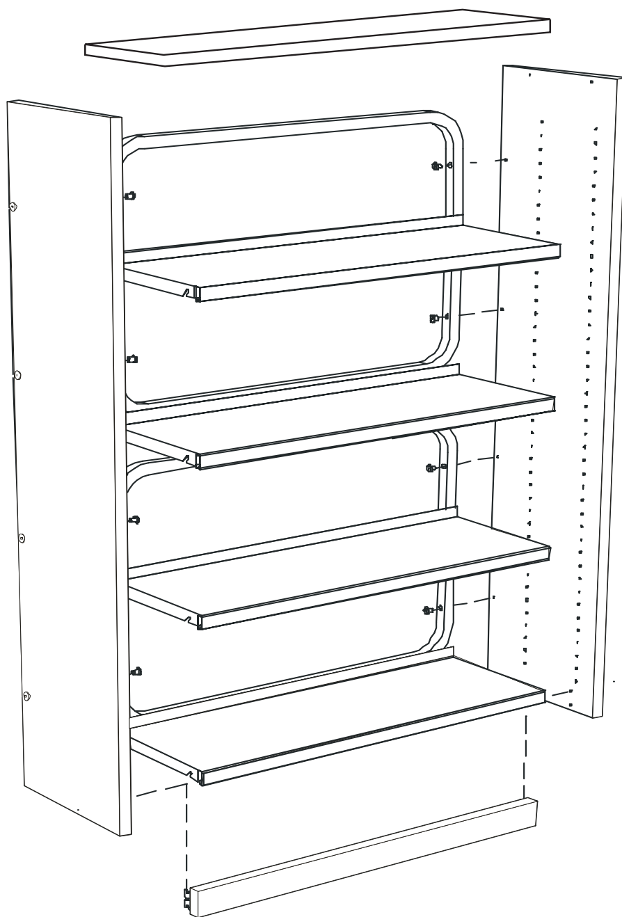
Typical Steel Frame Construction Bookcase Assembly
