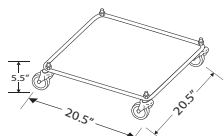
Bola, 4-wheel Dolly R00005
