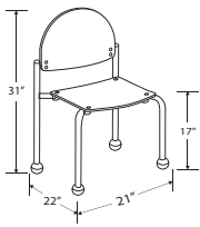
Bola, Rolled Front Leg, Fixed Back, Stacker, Armless BOL-R45018
