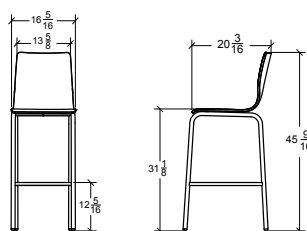
ROMAK Stool RMS2-30A
