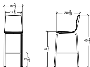
ROMAK Stool with Handle Grip RMS2-30A
